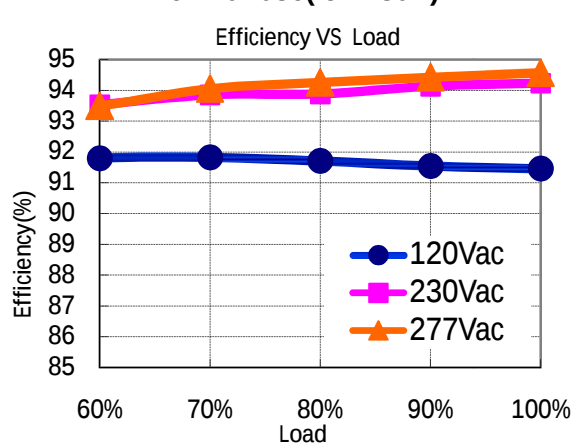
X6-240Y086 (Io=2.80A)
