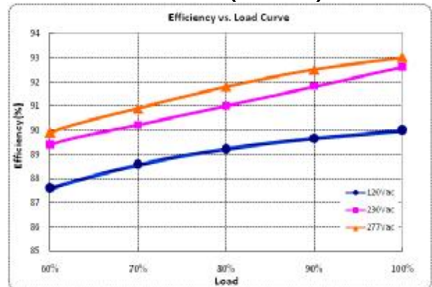
X6-240Y041 (Io=7.50A)
