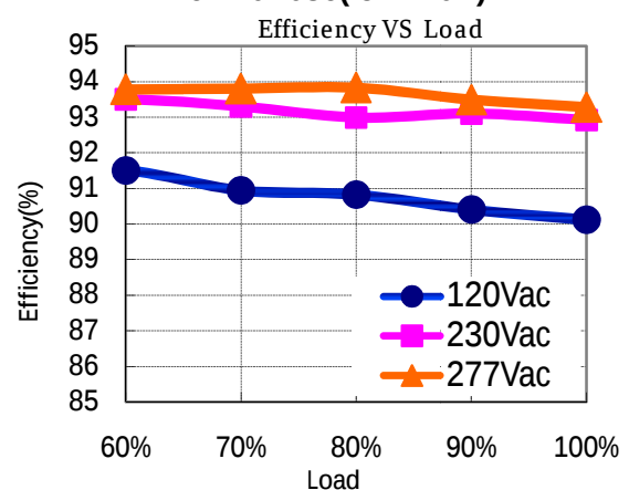
X6-240Y086 (Io=4.20A)
