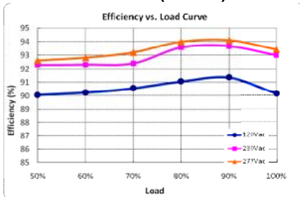
X6-240Y062 (Io=3.88A)
