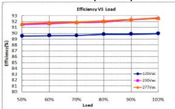
X6-105Y150 (Io=0.70A)
