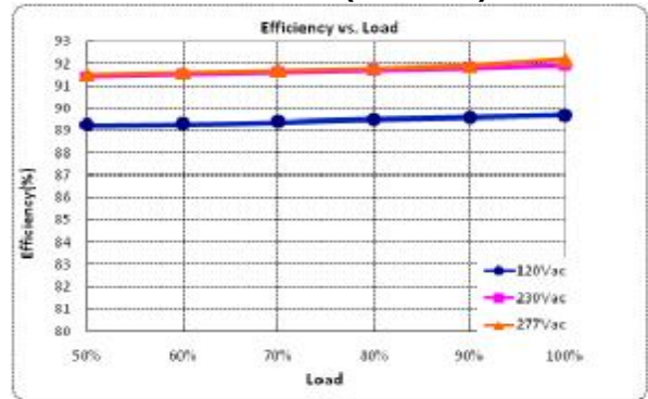
X6-105Y062 (Io=2.50A)
